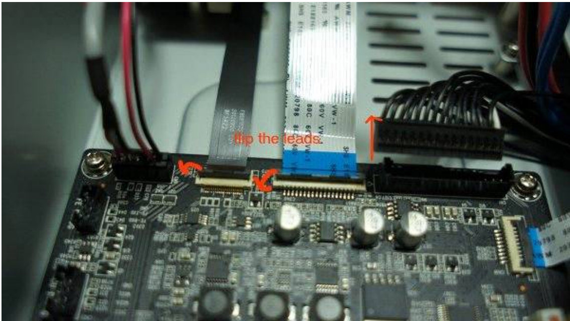
Flip the flat cable connector lid with finger and detach 15 pin power cable
