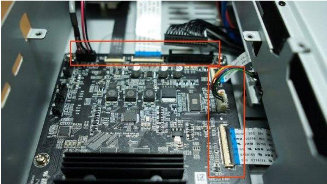
Flip the flat cable connector lid with finger and detach 15 pin power cable
